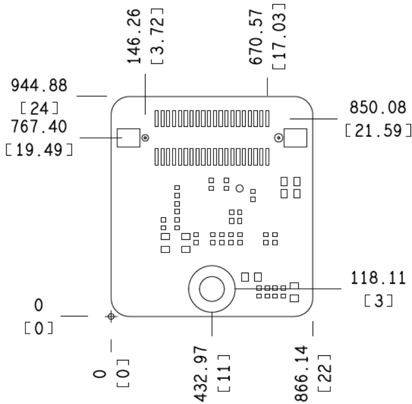
Figure 4: Mechanical outline of RGMII Board
